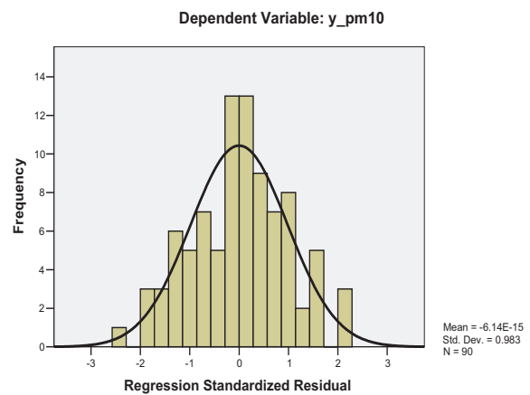
Fig. 2. Normality test
