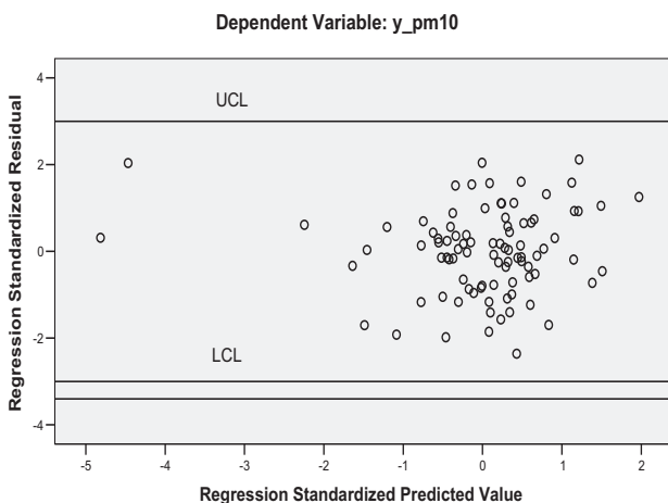
Fig. 1. Randomness test
